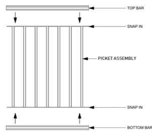
B) Snap Top & Bottom Bars onto Picket Assembly A)
